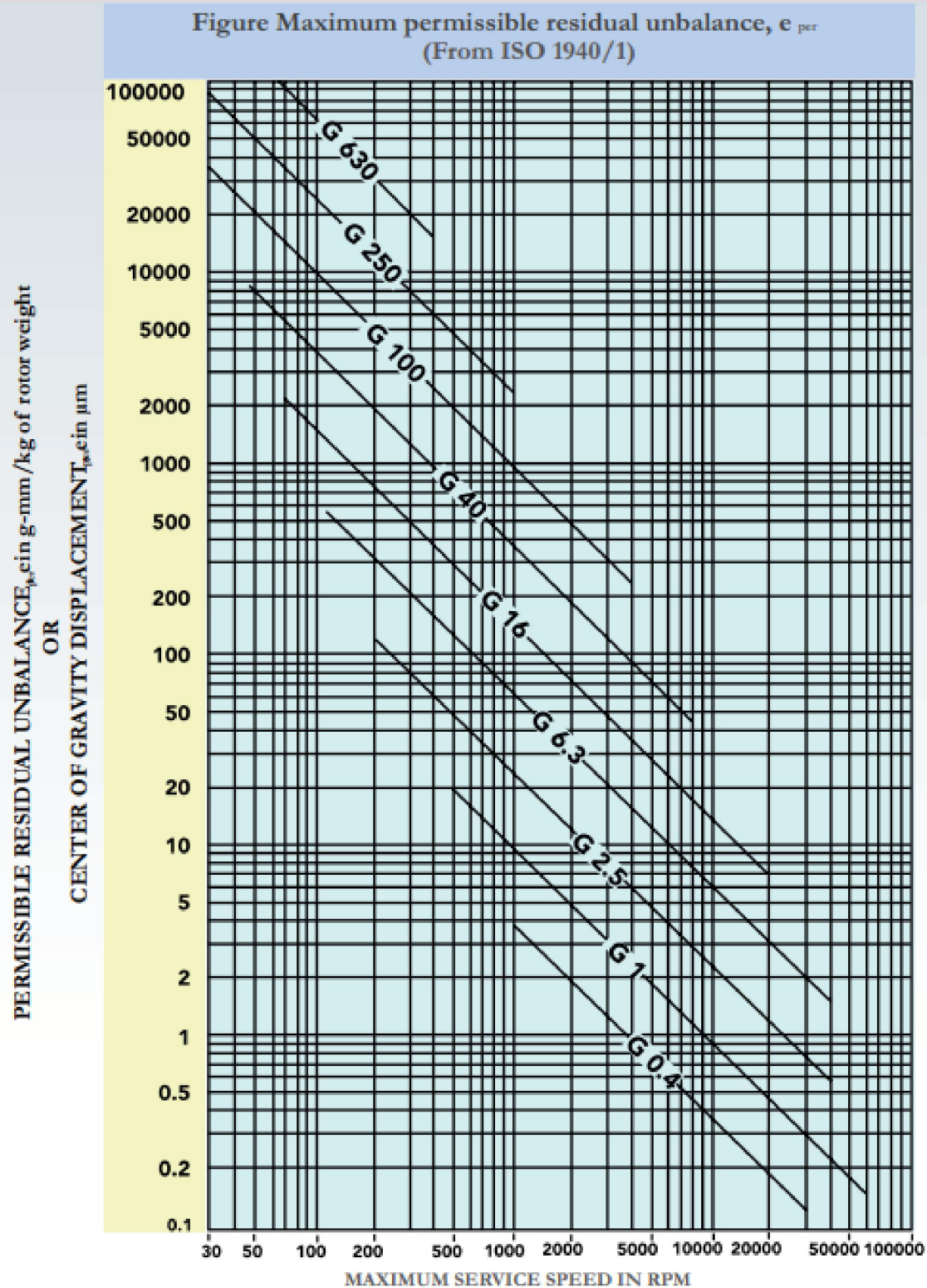
Figure : Maximum Permissible residual unbalance
