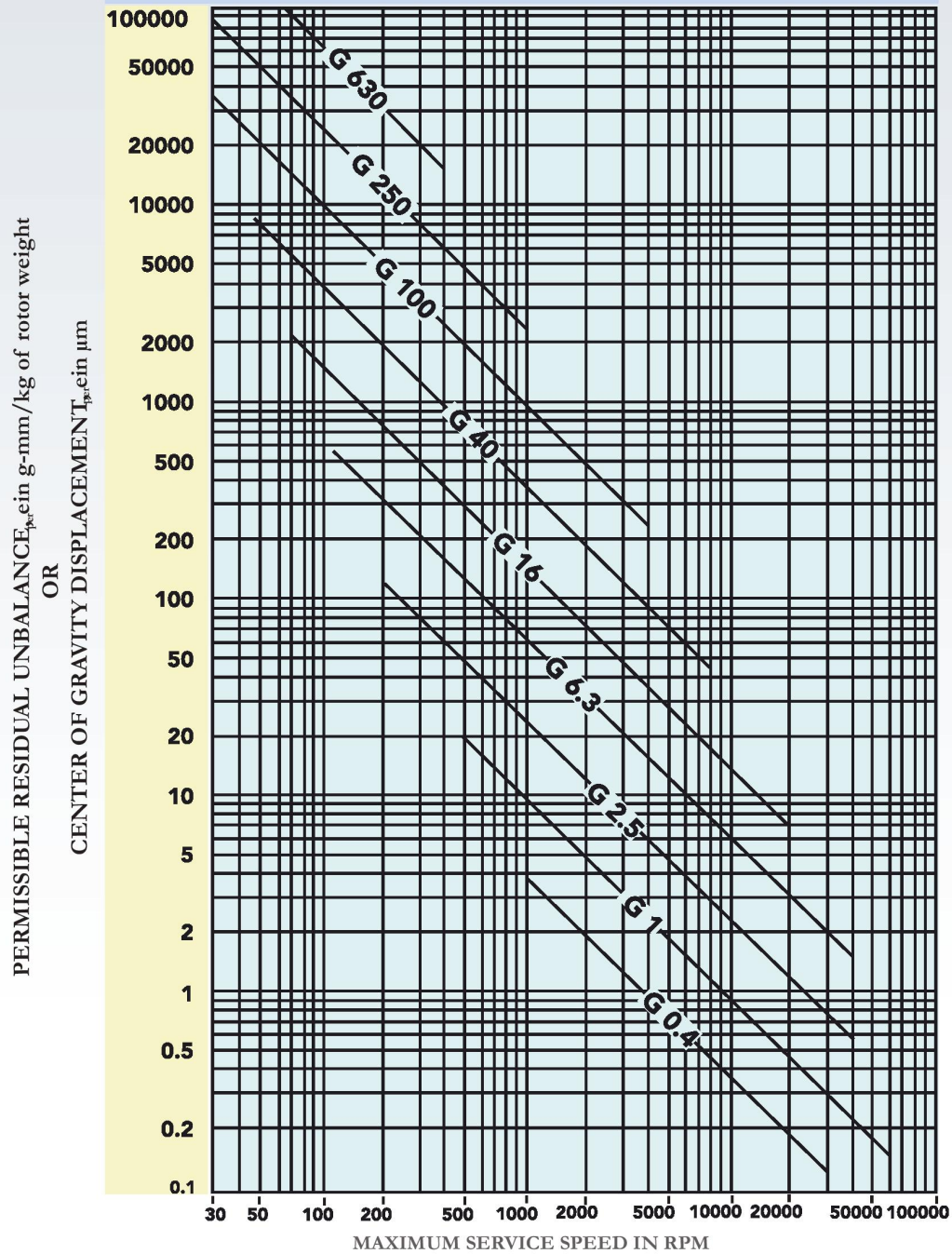
Figure Maximum permissible residual unbalance, e_{per} (From ISO 1940/1)
